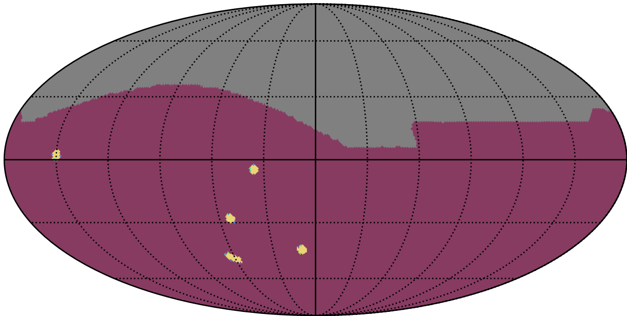
ddf_acor_sf20_lsf40_lsr10_v3.4_10yrs : NumberOfQuickRevisits
