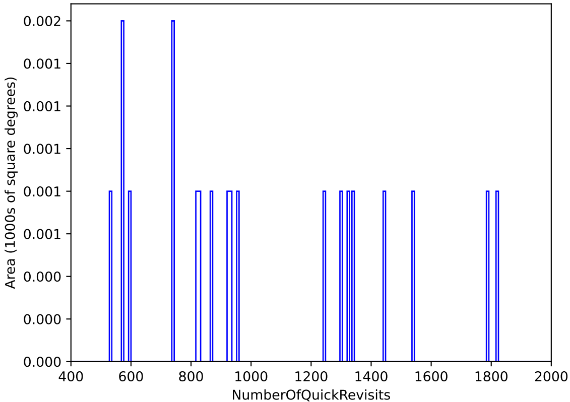
ddf_acor_sf20_lsf40_lsr10_v3.4_10yrs : NumberOfQuickRevisits
