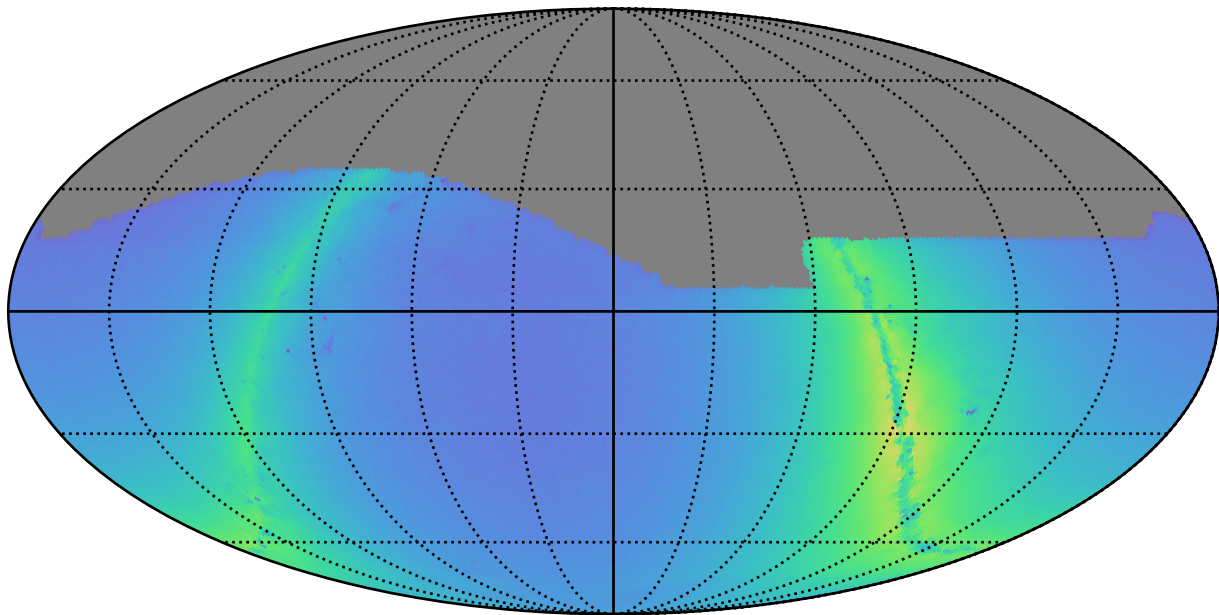
ddf_acor_sf20_lsf40_lsr10_v3.4_10yrs r: Nstars_no_crowding
