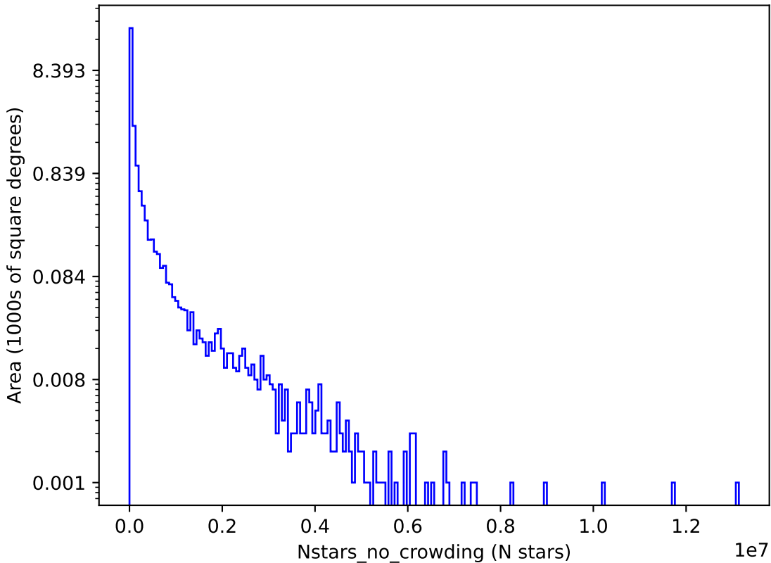
ddf_acor_sf20_lsf40_lsr10_v3.4_10yrs g: Nstars_no_crowding
