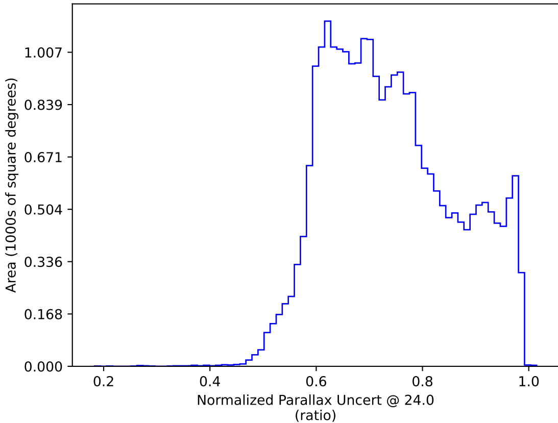
ddf_acor_sf20_lsf40_lsr10_v3.4_10yrs : Normalized Parallax Uncert @ 24.0
