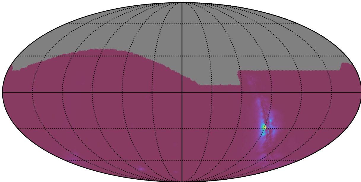
ddf_acor_sf20_lsf40_lsr10_v3.4_10yrs : NlcPoints
