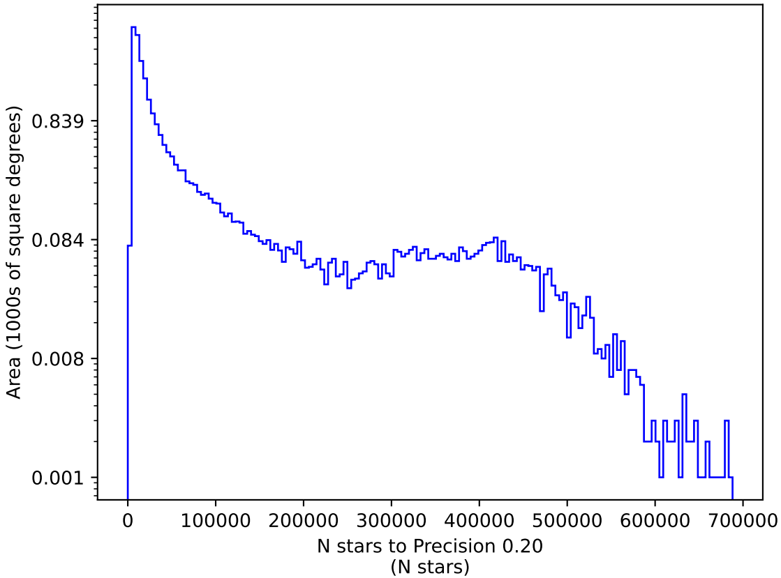
ddf_acor_sf20_lsf40_lsr10_v3.4_10yrs r: N stars to Precision 0.20
