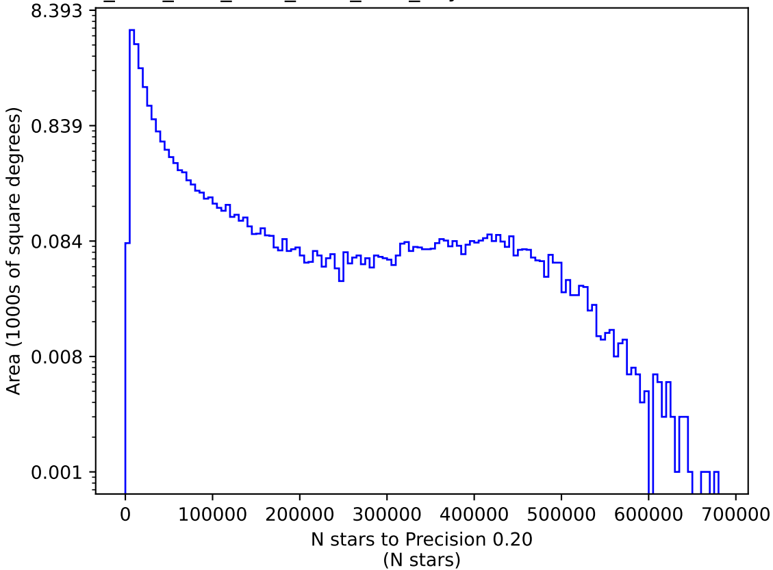
ddf_acor_sf20_lsf40_lsr10_v3.4_10yrs i: N stars to Precision 0.20
