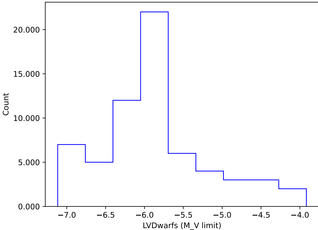
ddf_acor_sf20_lsf40_lsr10_v3.4_10yrs gi: LVDwarfs
