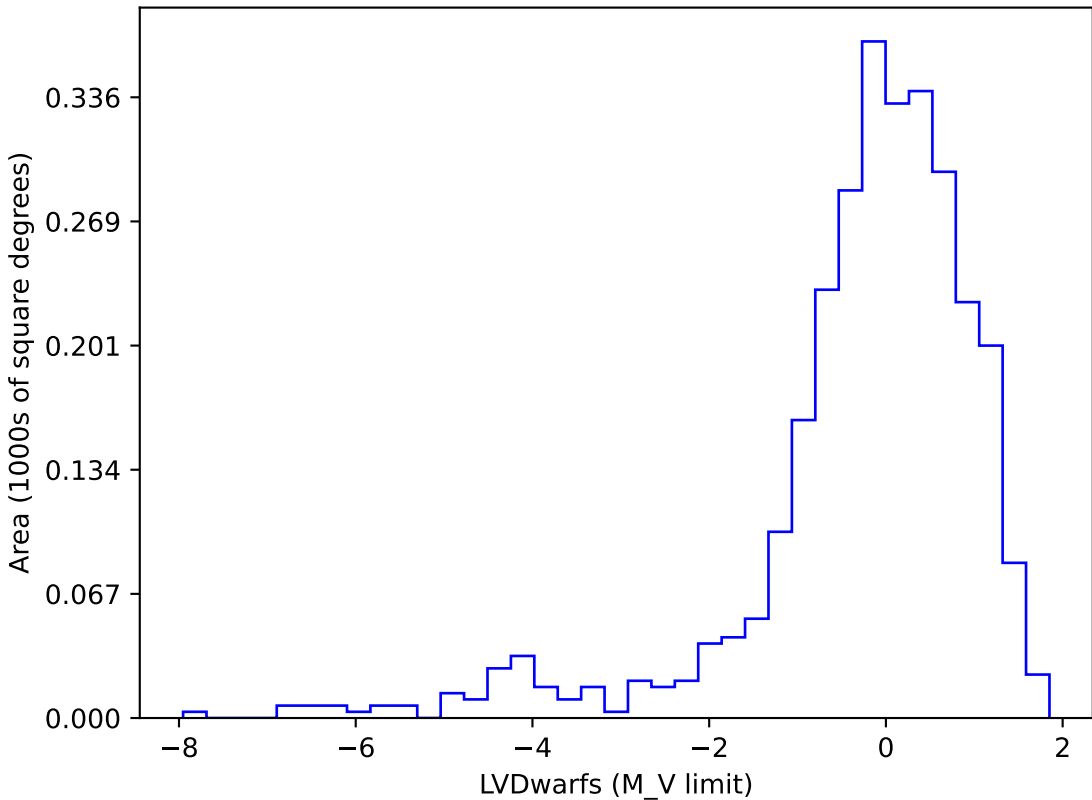
ddf_acor_sf20_lsf40_lsr10_v3.4_10yrs gi SCP: LVDwarfs
