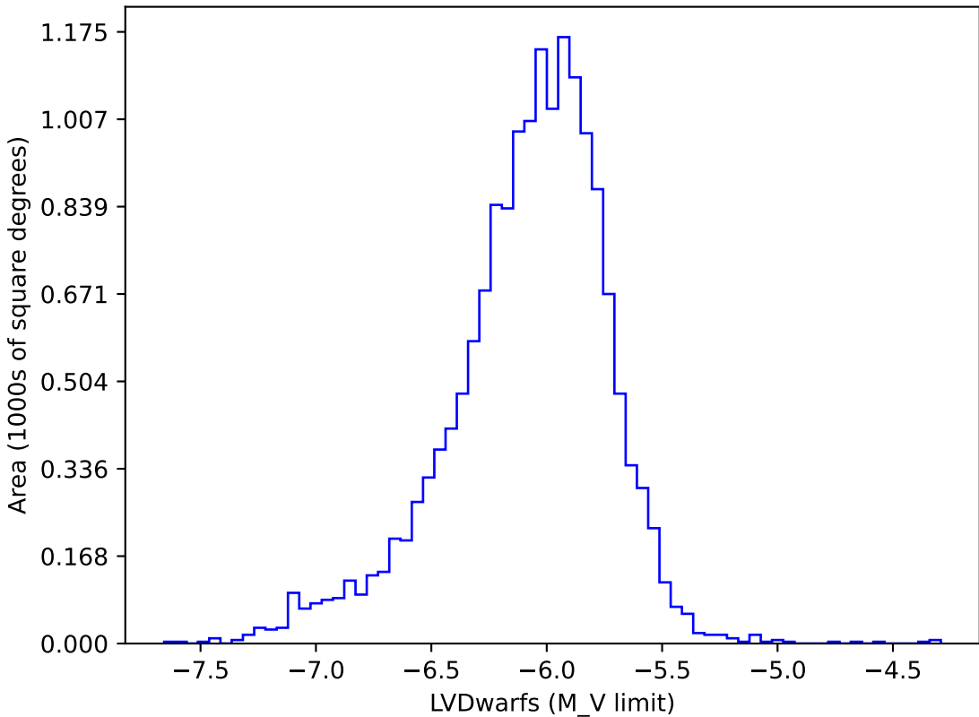
ddf_acor_sf20_lsf40_lsr10_v3.4_10yrs gi: LVDwarfs
