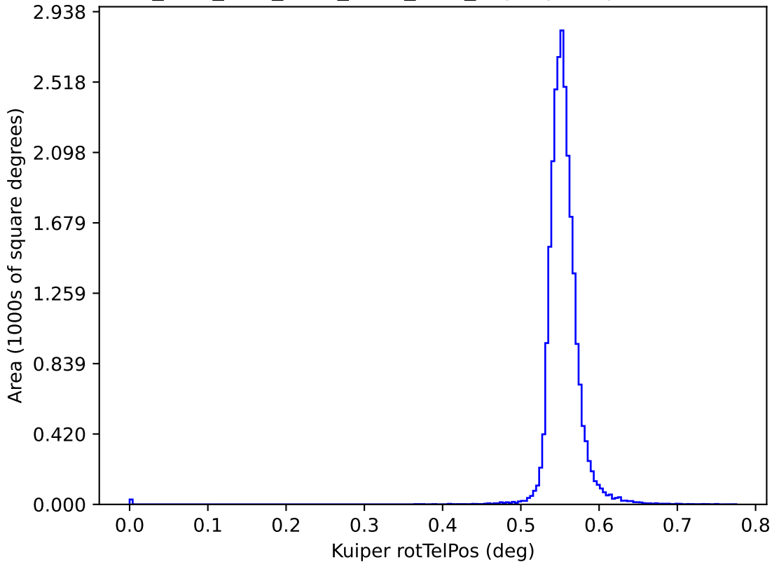
ddf_acor_sf20_ls40_lsr10_v3.4_10yrs y: Kuiper rotTelPos
