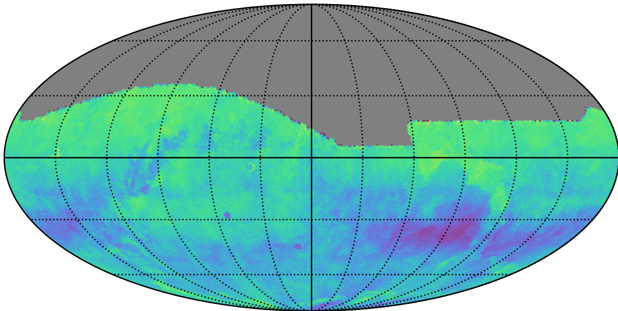
ddf_acor_sf20_lsf40_lsr10_v3.4_10yrs r: Kuiper rotSkyPos
