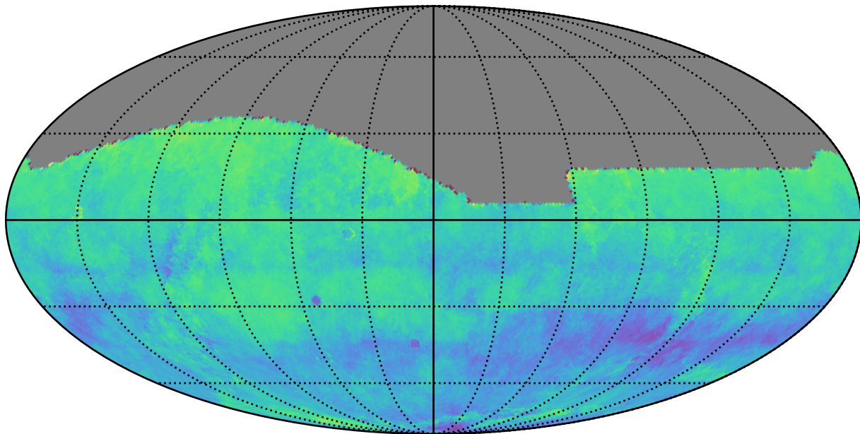
ddf_acor_sf20_lsf40_lsr10_v3.4_10yrs i: Kuiper rotSkyPos
