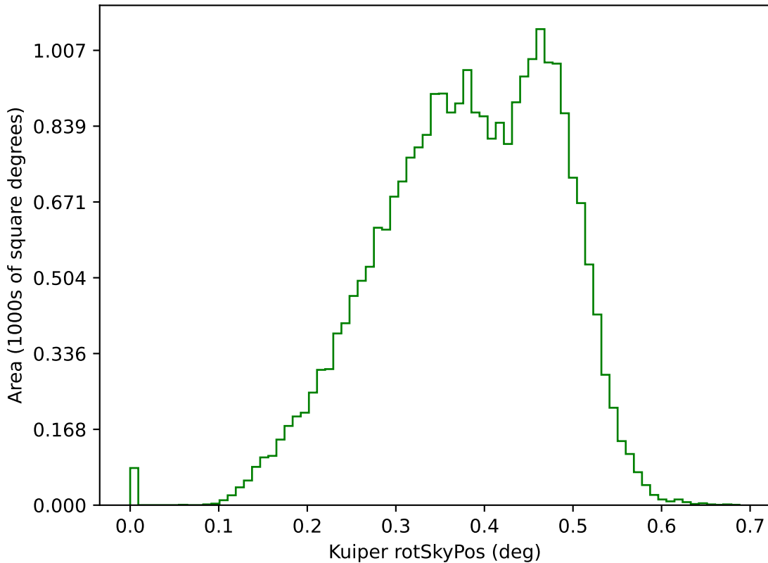
ddf_acor_sf20_lsf40_lsr10_v3.4_10yrs g: Kuiper rotSkyPos
