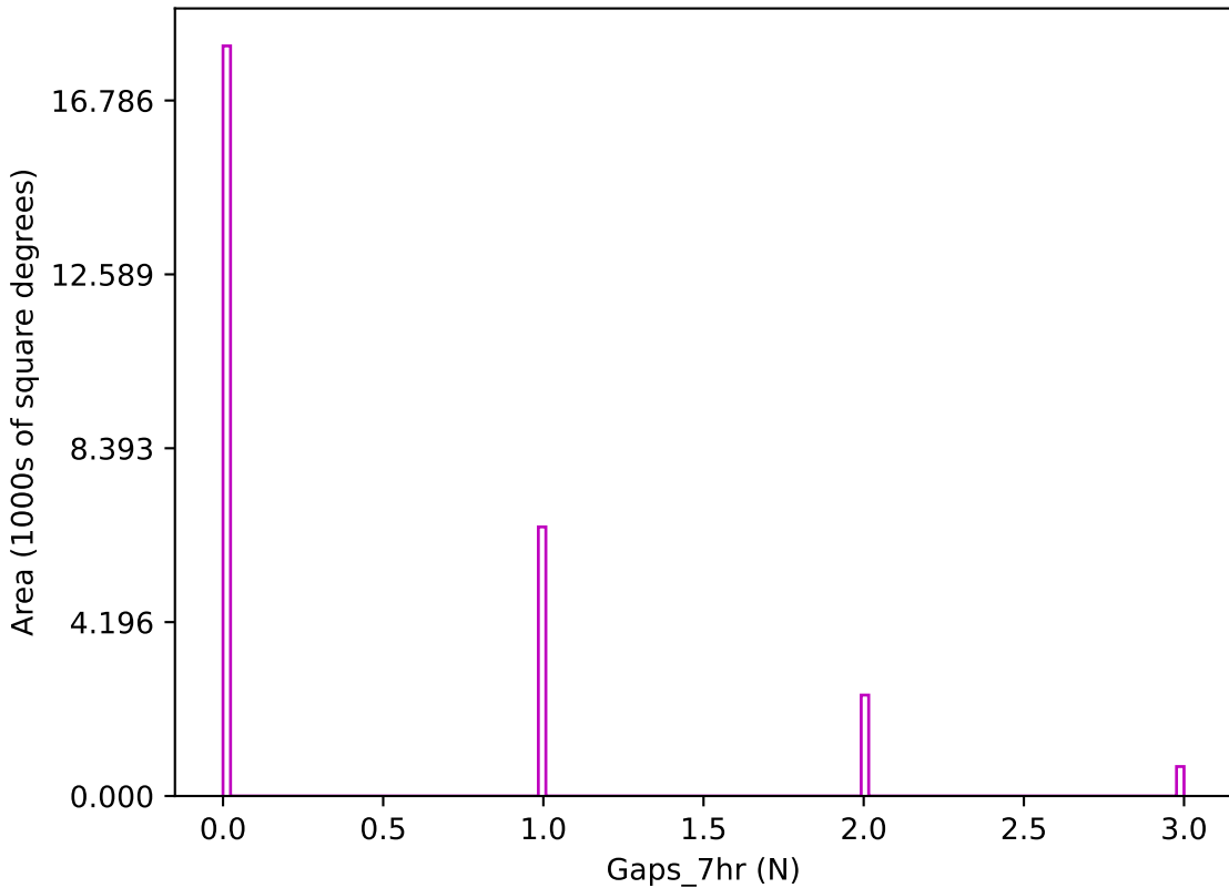
ddf_acor_sf20_lsf40_lsr10_v3.4_10yrs z band: Gaps_7hr
