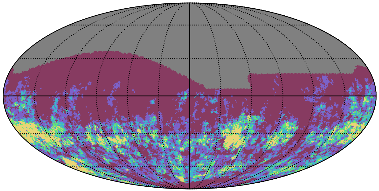
ddf_acor_sf20_lsf40_lsr10_v3.4_10yrs r band: Gaps_7hr
