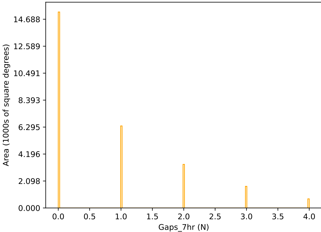
ddf_acor_sf20_lsf40_lsr10_v3.4_10yrs r band: Gaps_7hr
