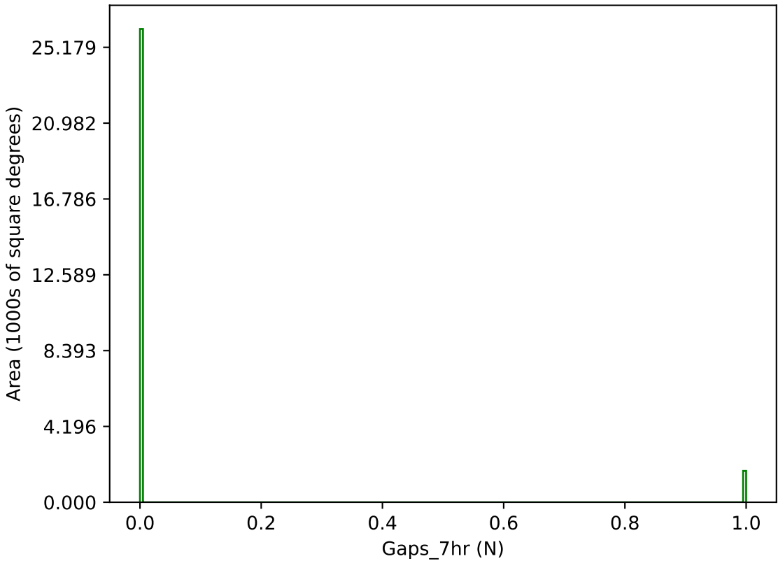
ddf_acor_sf20_lsf40_lsr10_v3.4_10yrs g band: Gaps_7hr
