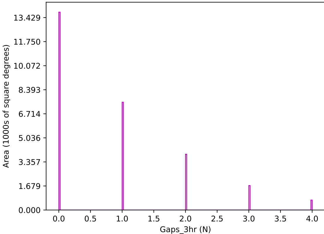
ddf_acor_sf20_lsf40_lsr10_v3.4_10yrs z band: Gaps_3hr
