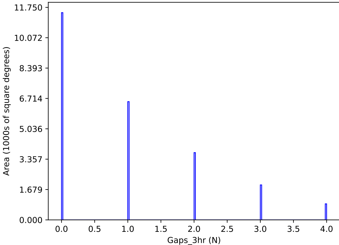
ddf_acor_sf20_ls40_lsr10_v3.4_10yrs y band: Gaps_3hr
