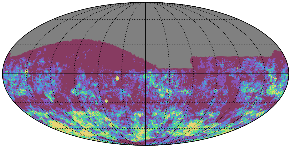
ddf_acor_sf20_lsf40_lsr10_v3.4_10yrs r band: Gaps_3hr
