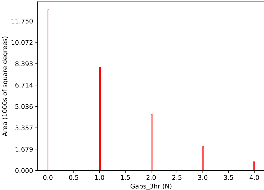
ddf_acor_sf20_lsf40_lsr10_v3.4_10yrs i band: Gaps_3hr
