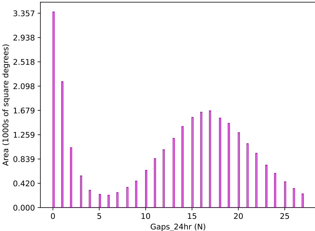
ddf_acor_sf20_ls40_lsr10_v3.4_10yrs z band: Gaps_24hr
