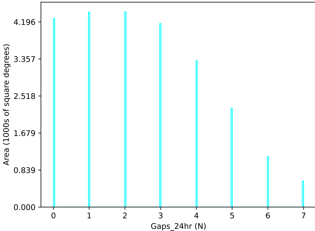
ddf_acor_sf20_lsf40_lsr10_v3.4_10yrs u band: Gaps_24hr
