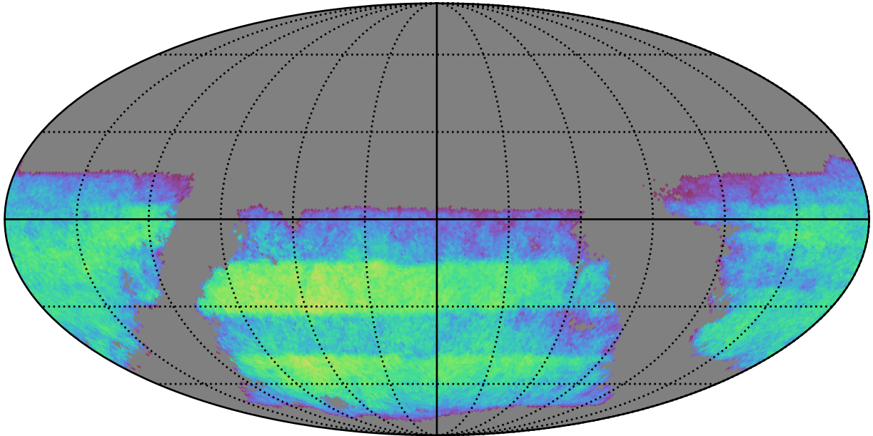
ddf_acor_sf20_lsf40_lsr10_v3.4_10yrs i band non-DD year 3: ExgalM5WithCuts
