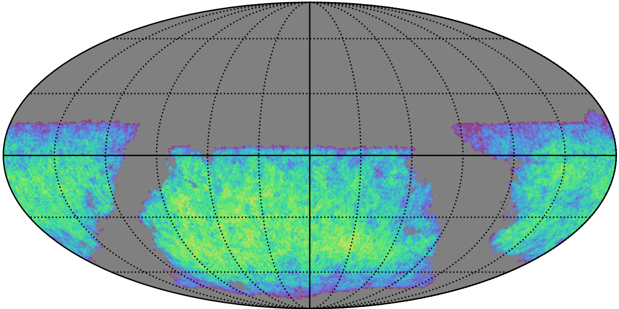
ddf_acor_sf20_lsf40_lsr10_v3.4_10yrs i band non-DD year 1: ExgalM5WithCuts
