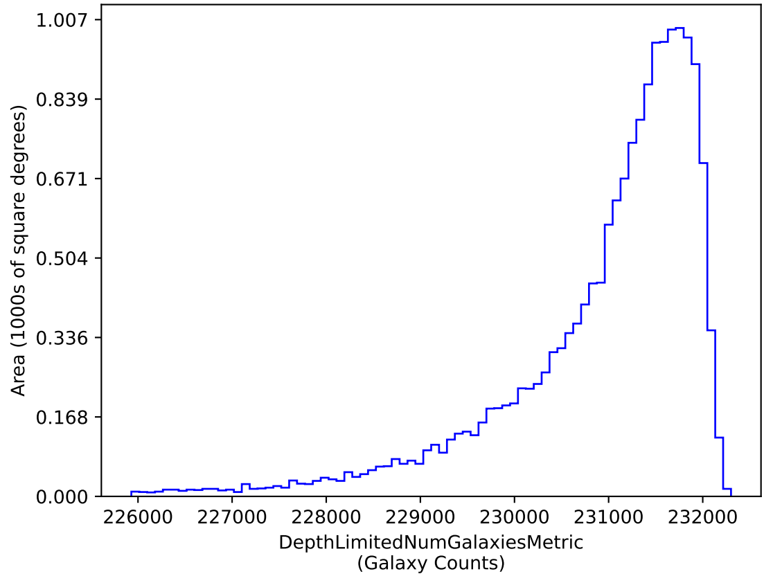
ddf_acor_sf20_lsf40_lsr10_v3.4_10yrs i band galaxies non-DD: DepthLimitedNumGalaxiesMetric
