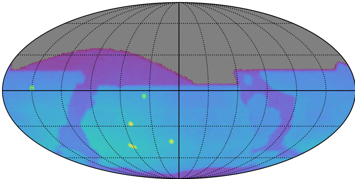
ddf_acor_sf20_lsf40_lsr10_v3.4_10yrs : Brown Dwarf, L4
