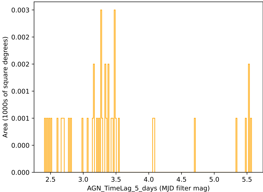
ddf_acor_sf20_lsf40_lsr10_v3.4_10yrs r band: AGN_TimeLag_5_days
