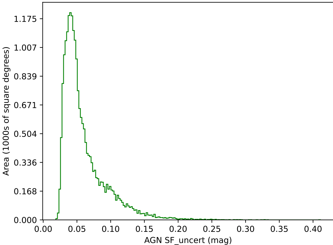
ddf_acor_sf20_lsf40_lsr10_v3.4_10yrs g band: AGN SF_uncert
