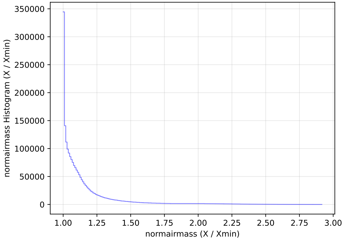
ddf_acor_sf20_lsf40_lsr10_v3.4_10yrs WFD all bands: normairmass Histogram
