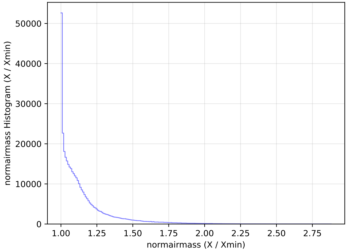
ddf_acor_sf20_lsf40_lsr10_v3.4_10yrs All sky y band: normairmass Histogram
