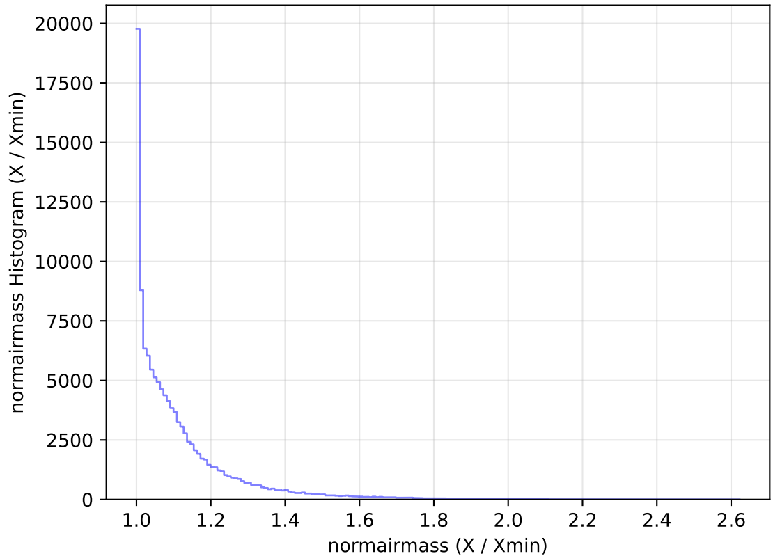
ddf_acor_sf20_lsf40_lsr10_v3.4_10yrs All sky u band: normairmass Histogram
