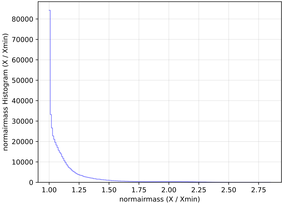
ddf_acor_sf20_lsf40_lsr10_v3.4_10yrs All sky r band: normairmass Histogram
