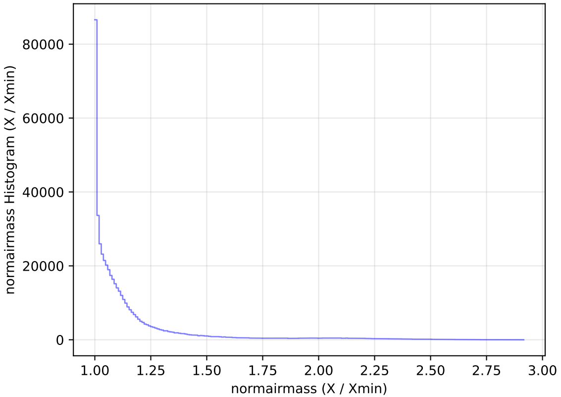
ddf_acor_sf20_lsf40_lsr10_v3.4_10yrs All sky i band: normairmass Histogram
