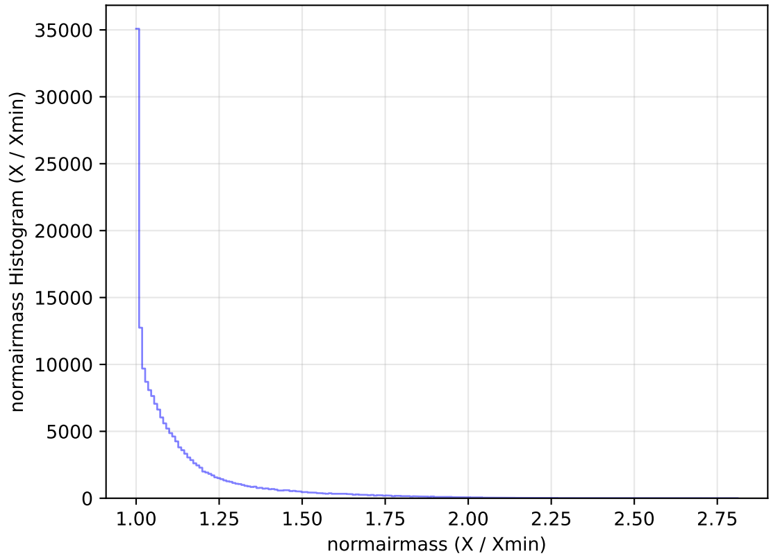
ddf_acor_sf20_lsf40_lsr10_v3.4_10yrs All sky g band: normairmass Histogram
