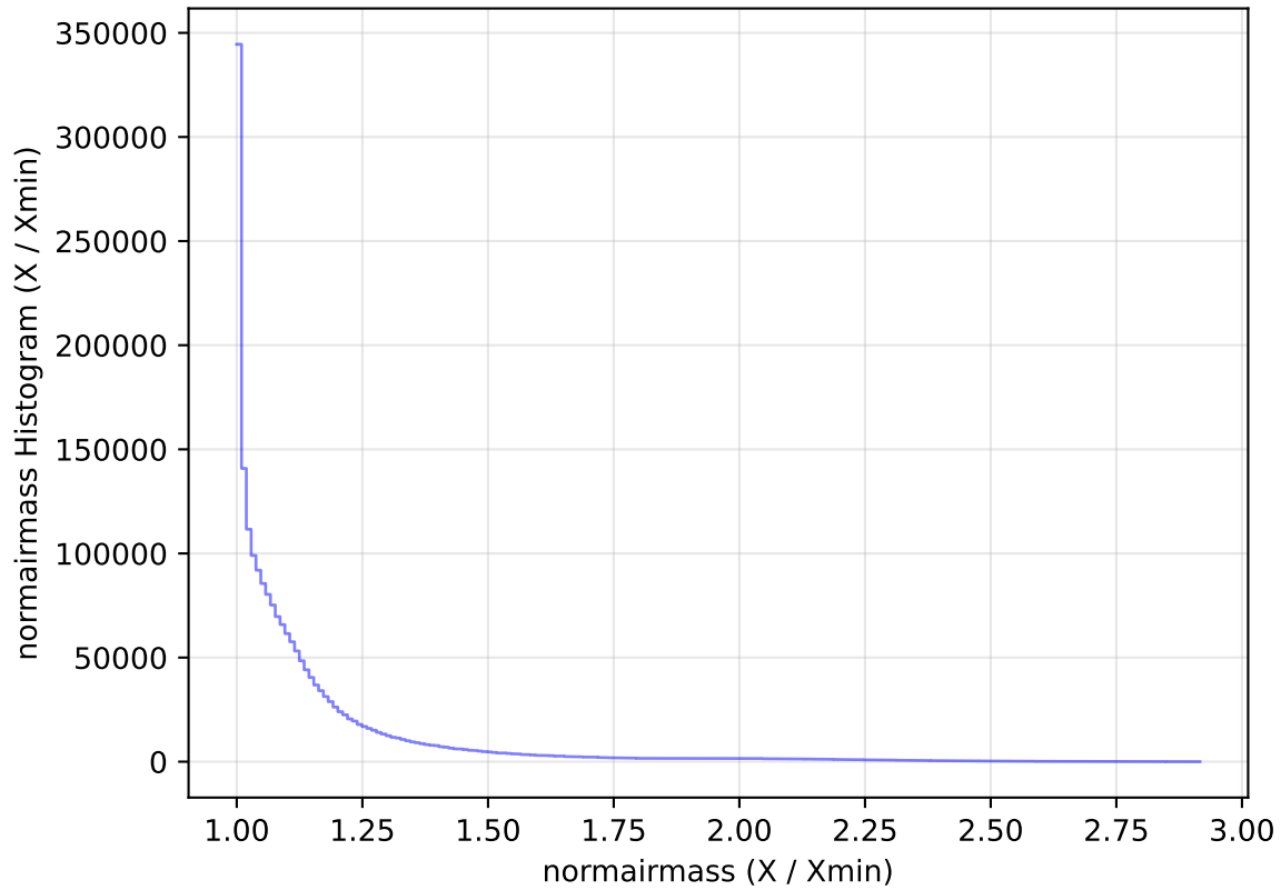
ddf_acor_sf20_lsf40_lsr10_v3.4_10yrs All sky all bands: normairmass Histogram
