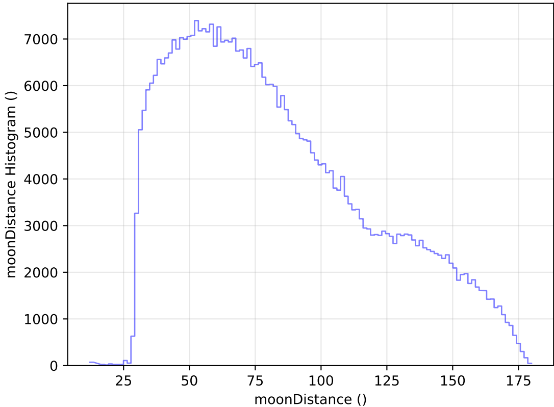
ddf_acor_sf20_Isf40_Isr10_v3.4_10yrs WFD z band: moonDistance Histogram
