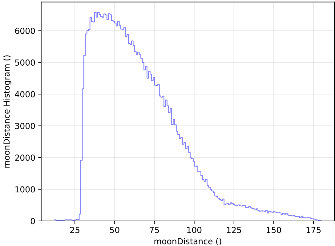
ddf_acor_sf20_Isf40_Isr10_v3.4_10yrs WFD y band: moonDistance Histogram
