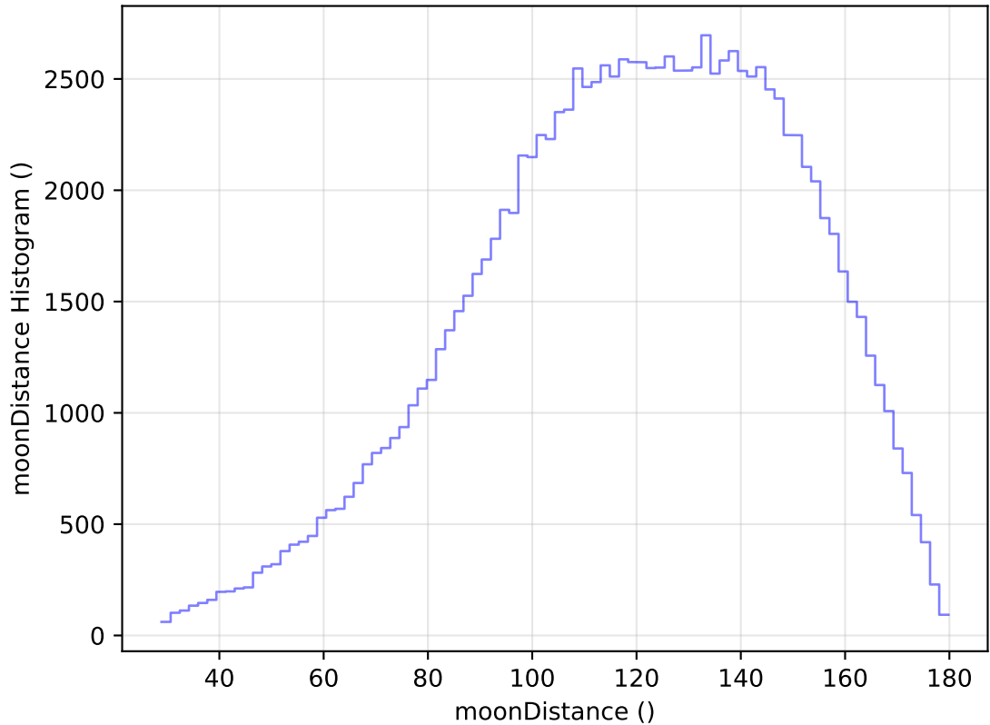
ddf_acor_sf20_lsf40_lsr10_v3.4_10yrs WFD u band: moonDistance Histogram
