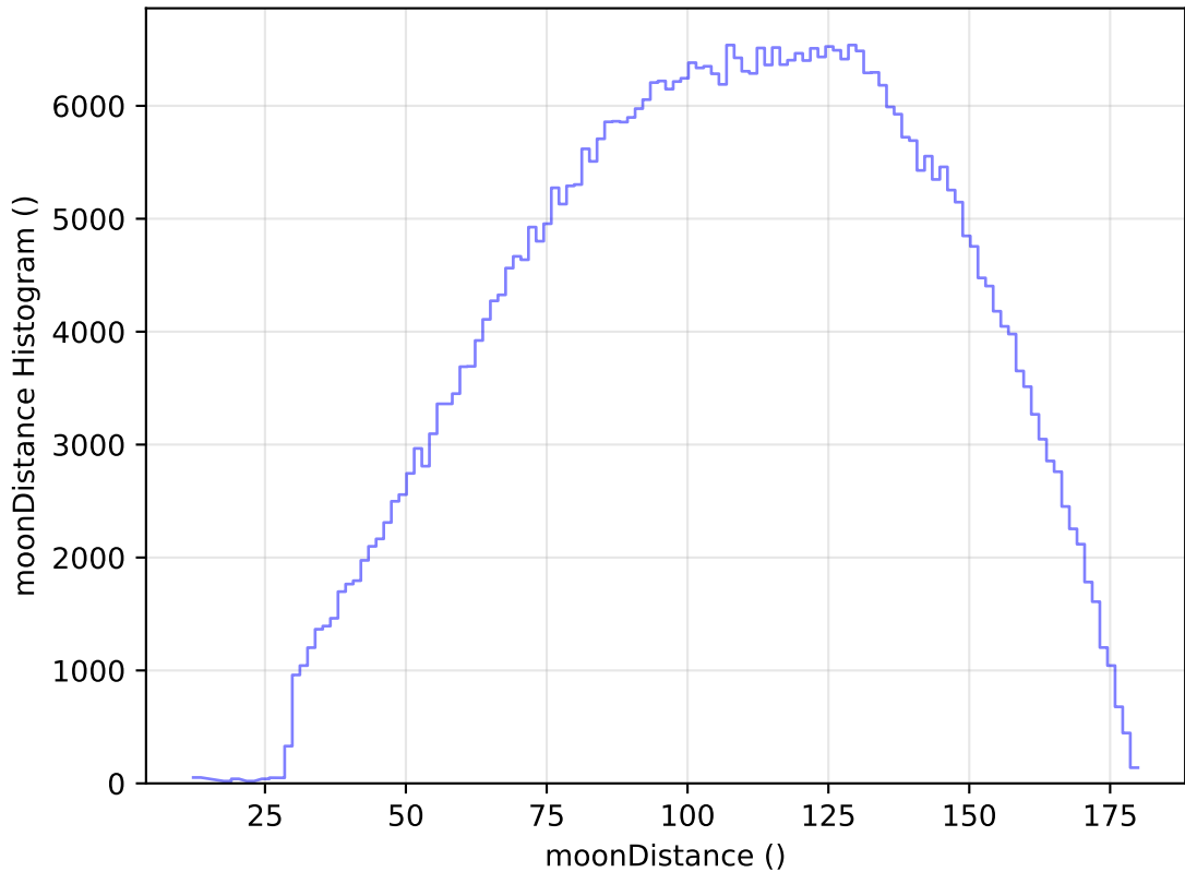
ddf_acor_sf20_lsf40_lsr10_v3.4_10yrs WFD r band: moonDistance Histogram
