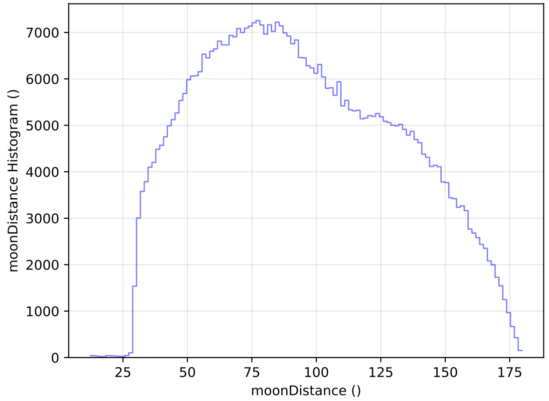
ddf_acor_sf20_lsf40_lsr10_v3.4_10yrs WFD i band: moonDistance Histogram
