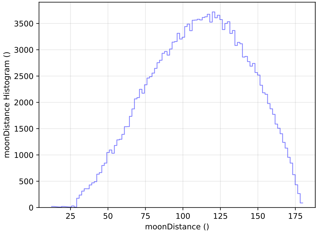
ddf_acor_sf20_lsf40_lsr10_v3.4_10yrs WFD g band: moonDistance Histogram
