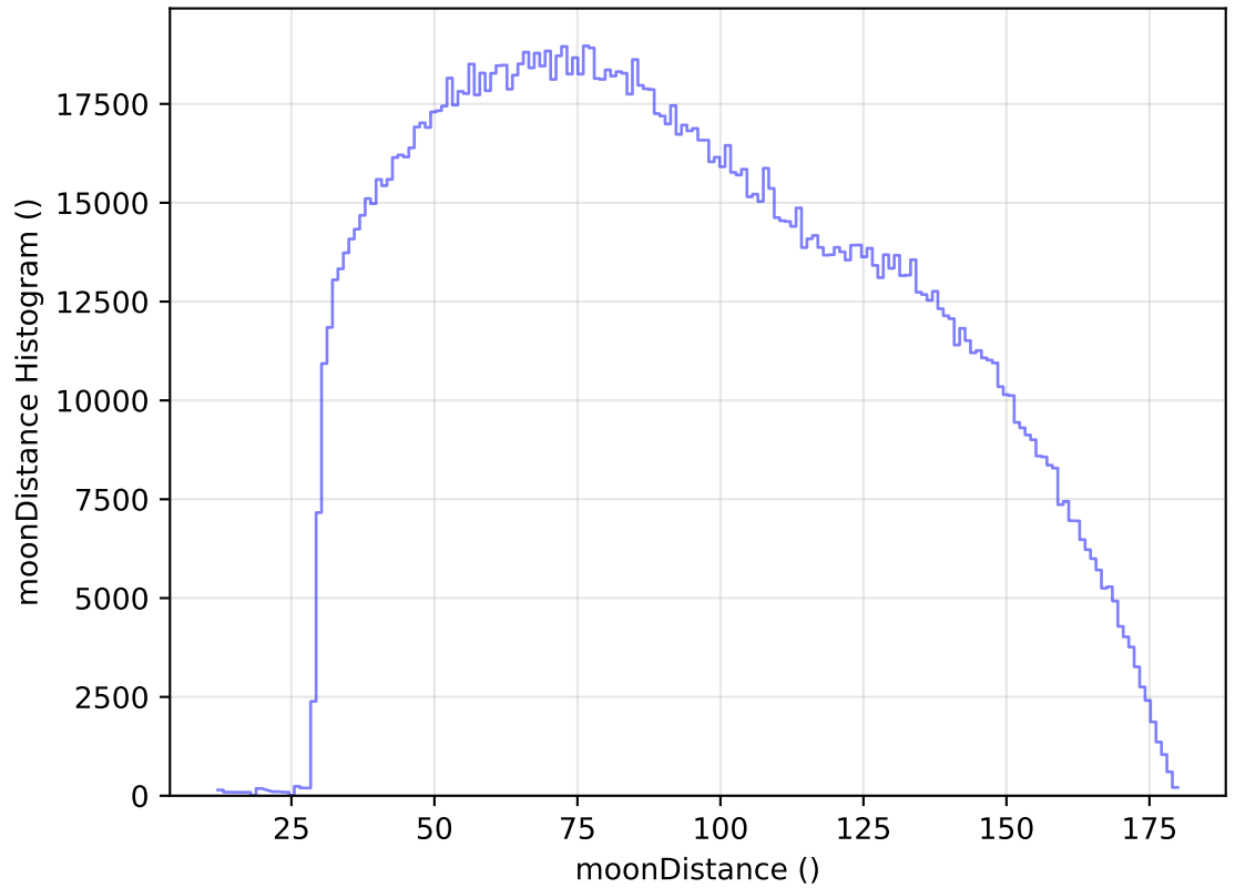
ddf_acor_sf20_lsf40_lsr10_v3.4_10yrs WFD all bands: moonDistance Histogram
