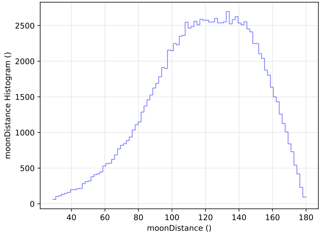
ddf_acor_sf20_lsf40_lsr10_v3.4_10yrs All sky u band: moonDistance Histogram
