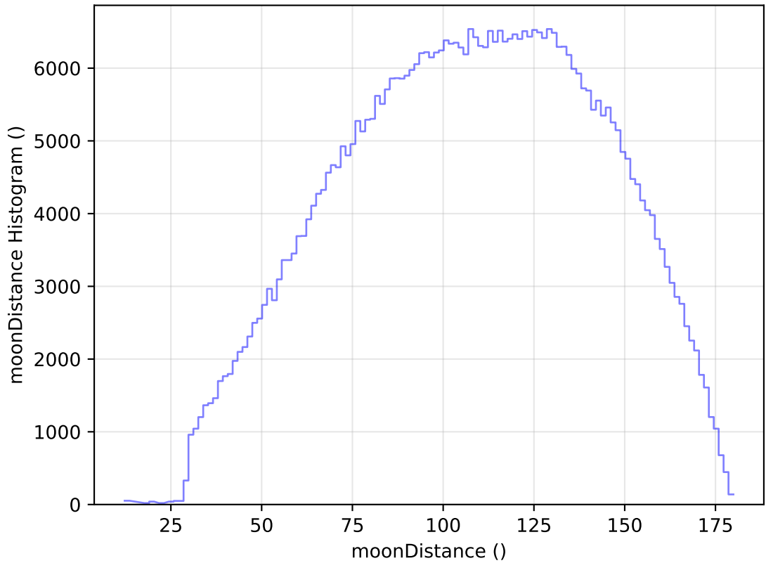
ddf_acor_sf20_lsf40_lsr10_v3.4_10yrs All sky r band: moonDistance Histogram
