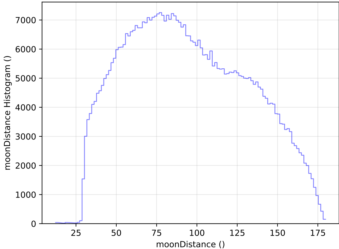
ddf_acor_sf20_lsf40_lsr10_v3.4_10yrs All sky i band: moonDistance Histogram
