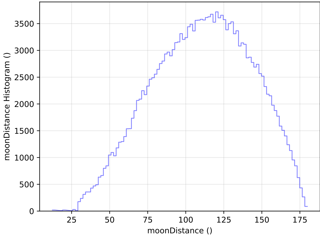
ddf_acor_sf20_lsf40_lsr10_v3.4_10yrs All sky g band: moonDistance Histogram
