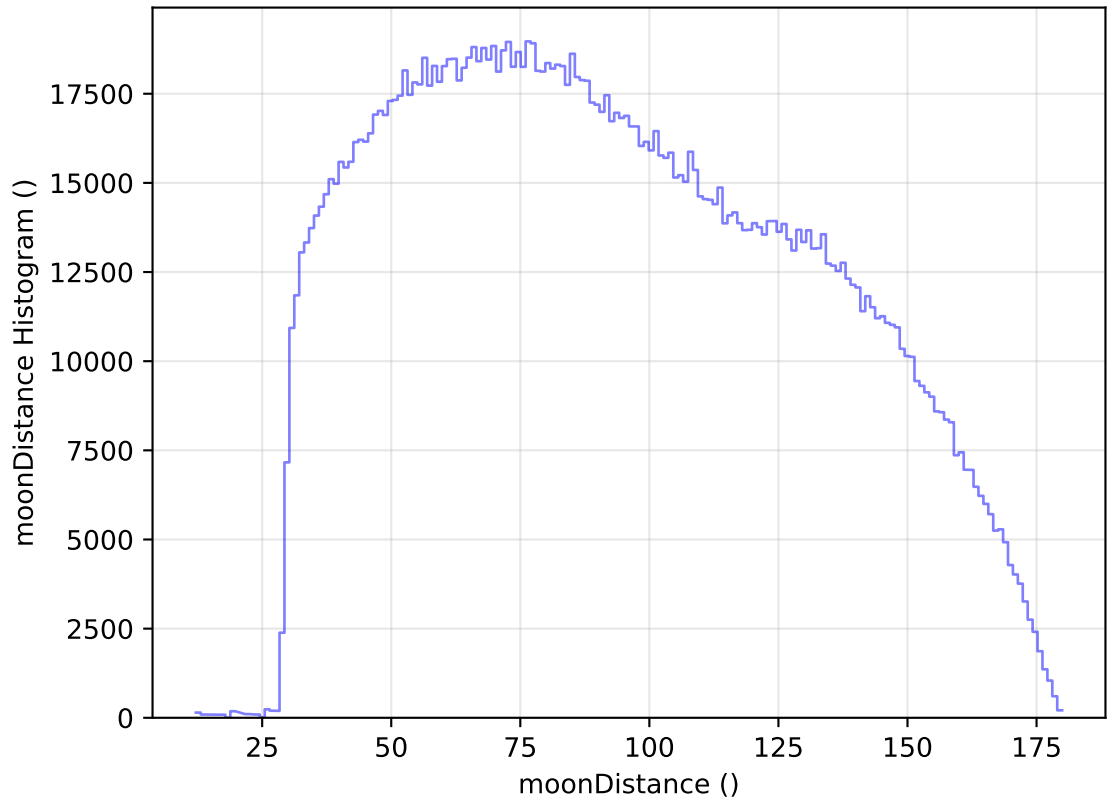
ddf_acor_sf20_lsf40_lsr10_v3.4_10yrs All sky all bands: moonDistance Histogram
